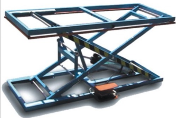
TAVOLO ELEVATORE MOD. STX-10 LIFTABLE TABLE MOD. STX-10
